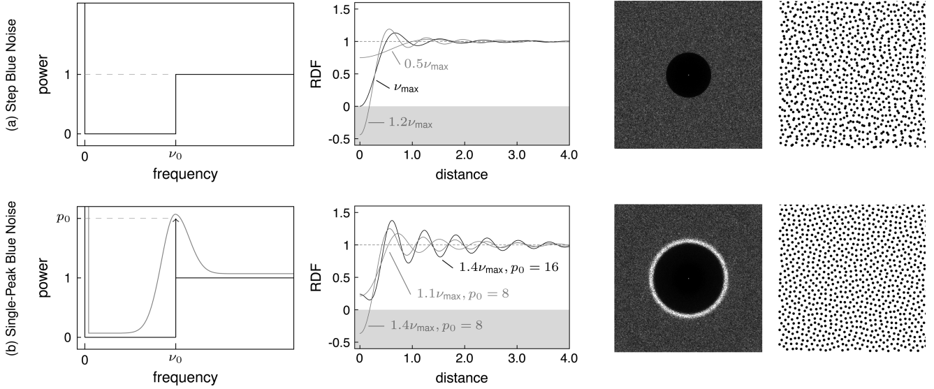
Fig. 4. Radial power spectra, corresponding RDFs, two-dimensional power spectra and cutouts from corresponding points sets for step blue noise and single-peak blue noise. (a) A radial power spectrum that is a perfect step is only possible up to a maximum frequency \nu_{\max} . For frequencies \nu_0 > \nu_{\max} the corresponding RDF becomes negative. (b) To achieve a higher effective Nyquist frequency, we have to allow the power spectrum to go above 1 by introducing a (potentially smoothed) peak around \nu_0 > \nu_{\max} . To keep the corresponding RDF positive, we have to increase the height p_0 of the peak as we increase \nu_0 .
