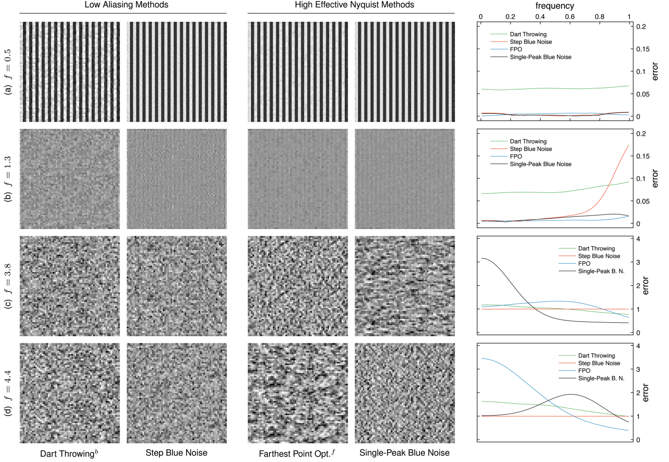
Fig. 7. Illustration of the sampling error for sinusoids of increasing frequencies. The plots in the rightmost column show the predicted frequency distribution of the noise in the shown images. The frequency axis is relative to v_{px} , the Nyquist frequency of the pixel grid. Note how the shape of the error curve corresponds to noise in the image: flat curves show up as white noise, whereas peaks in the curve lead to different forms of colored noise.
