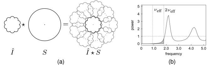
Fig. 3. (a) The spectrum of the sampled signal \hat{I}_s is obtained by convolving the original spectrum with the Fourier transform of the sampling pattern. Aliasing occurs when the replicated spectra \hat{I} overlap the central spectrum on the right-hand side. (b) The effective Nyquist frequency is a measure for the size of the zero region in the power spectrum. It is chosen so that 2v_{\text{eff}} roughly corresponds to the radius of the circle representing S in (a).
