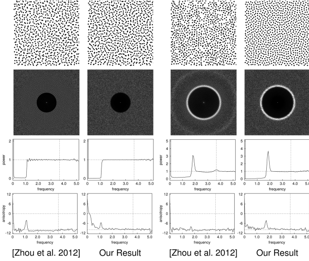
Fig. 6. Comparison of matching P_{\text{step}} (left) and P_{\text{peak}} (right) using the method by Zhou et al. [2012] and our approach. Our method matches the target power spectra slightly better and does not show defects in the underlying point distributions. For both methods, the anisotropy shows a noticeable response at the frequency of the step in the corresponding power spectrum.
