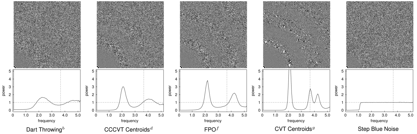
Fig. 1. A bird's eye view of the standard zone plate reveals structured aliasing for blue noise patterns that have peaks in their power spectrum. High-frequency image content is not replaced by white noise (as is the goal of stochastic sampling) but by pseudo-patterns that are conceptually similar to the moiré patterns of regular sampling. Step blue noise patterns, as defined in Section 3.1, consistently prevent such artifacts by cleanly mapping all high frequencies to white noise. (The superscripts refer to the citations in Table 1.)
