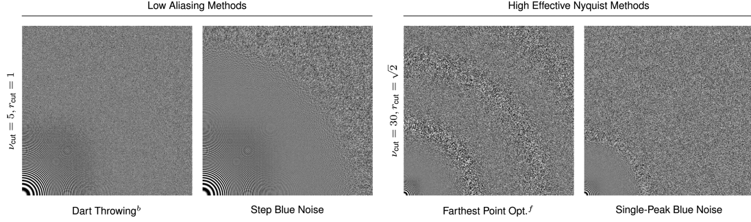
Fig. 8. A closer look at the behavior of step and single-peak blue noise patterns when used for image-plane sampling. (Left) Like dart throwing, step blue noise produces almost no structured aliasing, but it also keeps low-frequency content much cleaner. (Right) Like traditional blue noise patterns, single-peak blue noise can produce structured aliasing, but only for a narrow range of frequencies around 2\nu_{\text{eff}} . Lower frequencies are represented just as cleanly.
