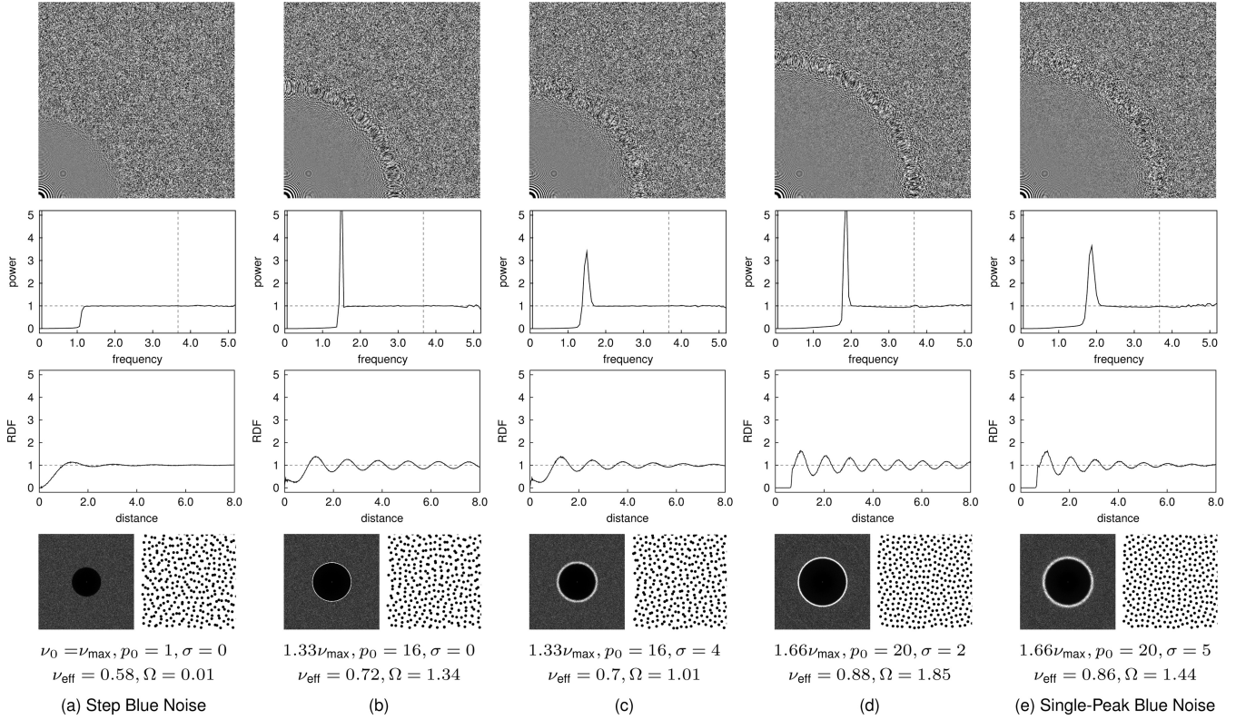
Fig. 5. A selection of realizable blue noise patterns with a single peak. (a) Step blue noise with a step of constant power and \nu_{\text{eff}} = 0.58 . (b) We can increase \nu_{\text{eff}} by moving energy to higher frequencies—in this case a Dirac peak of height P(\nu_0) = 16 —but only at the cost of structured aliasing (visible patterns in the form of rings around \nu_0 ). (c) Smoothing the peak to P(\nu_0) \approx 4 yields acceptable aliasing at the cost of a slightly reduced \nu_{\text{eff}} . (d) The highest effective Nyquist frequency we can produce without deviating strongly from a flat spectrum in frequencies below or above \nu_0 . (e) The best compromise we found between a high \nu_{\text{eff}} and structured aliasing. The stated parameters are for 4096 points; for other sizes n , the parameters p_0 and \sigma must be scaled by \sqrt{n/4096} .
