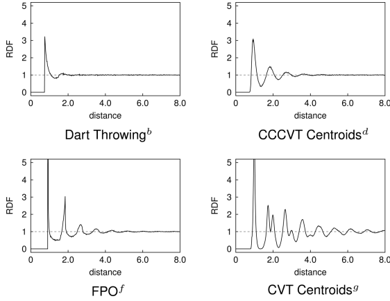
Fig. 2. Radial distribution functions for several of the blue noise patterns in Figure 1.
